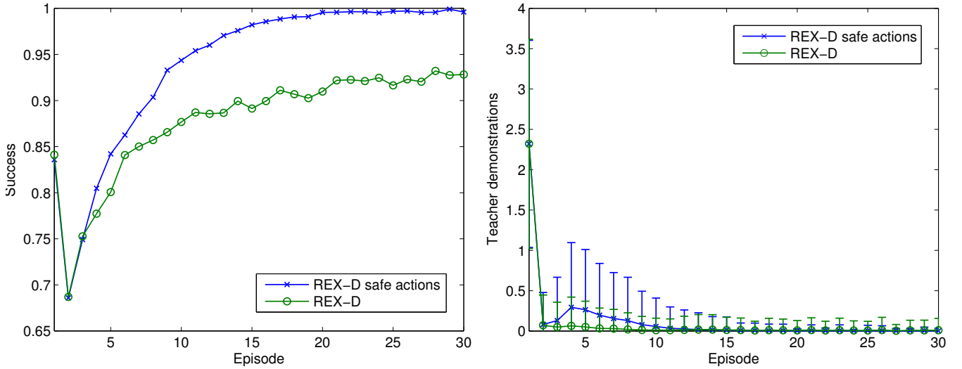
Fig. 2. Results in the Triangle Tireworld domain. The mean and standard deviations obtained over 2500 runs are shown. The exploration threshold is \zeta = 2 . Left: the success ratio of the algorithms. Right: the number of teacher demonstrations requested.
