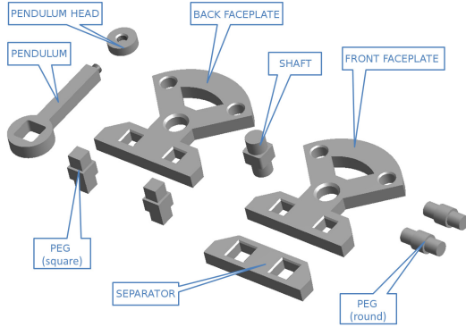
Fig. 3. Cranfield benchmark assembly. To assemble it, the different parts have to be placed in a restricted order: the separator requires the square pegs to be placed, the pendulum must be placed after the shaft, and the front faceplate requires all pegs, the separator and the pendulum to be in place.
