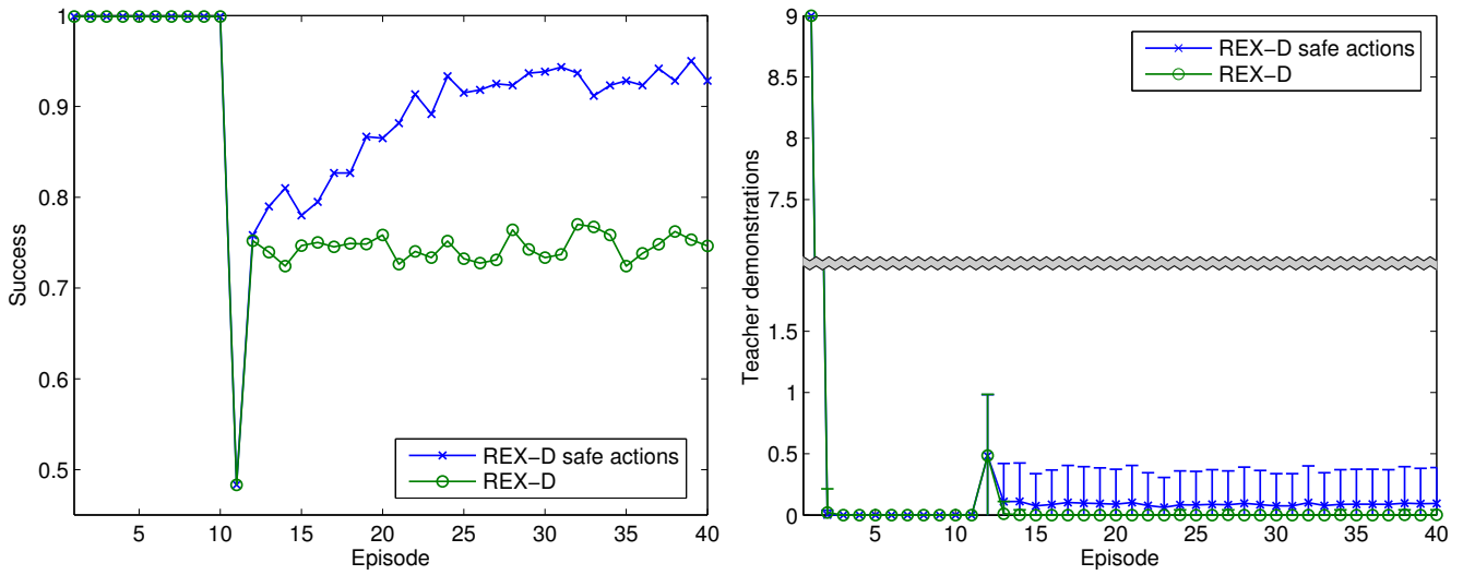
Fig. 4. Results in the Cranfield benchmark scenario. The mean and standard deviations obtained over 500 runs are shown. The exploration threshold is \zeta = 2 . During the 10 first episodes, all pegs start in a standard vertical position, and after the 11 th episode a peg is always positioned laying horizontally on the table. Left: the success ratio of the algorithms. Right: the number of teacher demonstrations requested.
